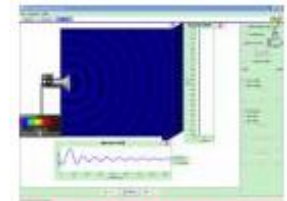
Wave Interference
